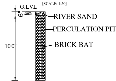
PERCOLATION PIT
