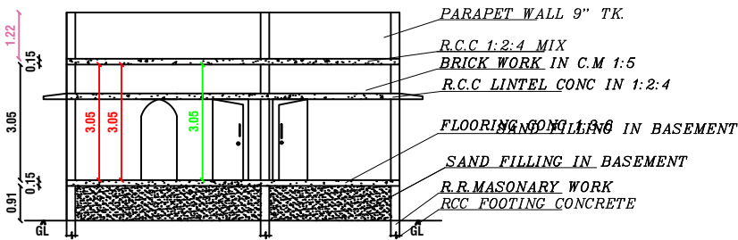
SIDE SECTION "AA"
