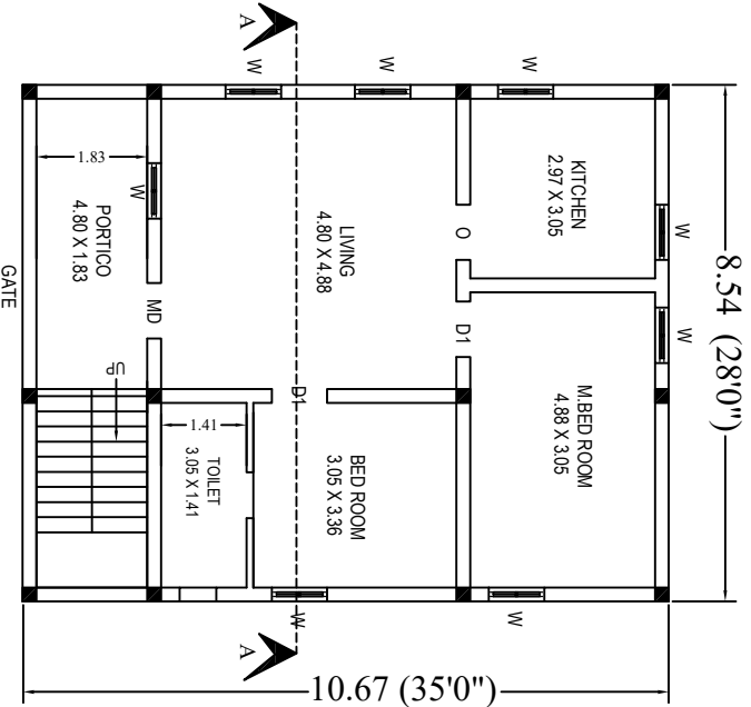
PRO.GROUND FLOOR
