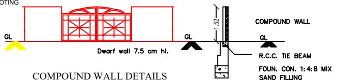
COMPOUND WALL DETAILS
