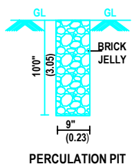
PERCOLATION PIT
