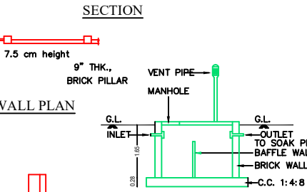
SECTION OF SEPT.TANK
