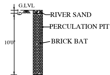
PERCOLATION PIT
