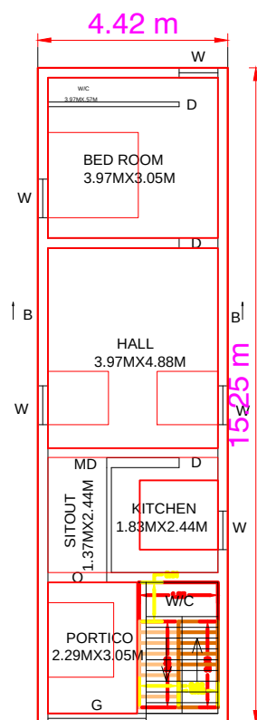
FIRST FLOOR(Pro.)
