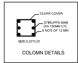
COLUMN DETAILS
