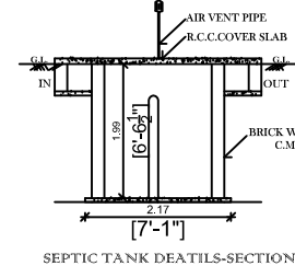
SEPTIC TANK DETAILS-SECTION
