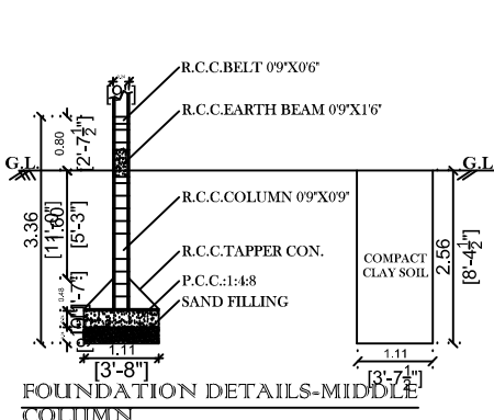
FOUNDATION DETAILS-MIDDLE COLUMN
