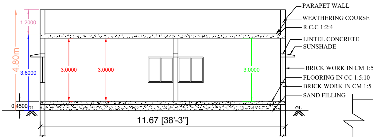
SECTION AB
