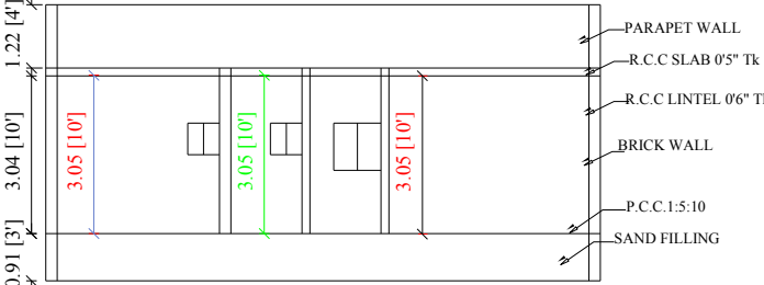
SECTION ON"AB"
