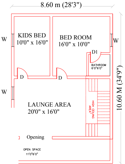
PRO.FIRST FLOOR
