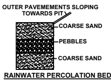
RAINWATER PERCOLATION BED
