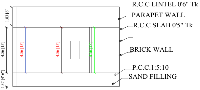
SECTION ON"AB"
