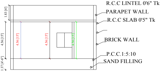
SECTION ON"AB"
