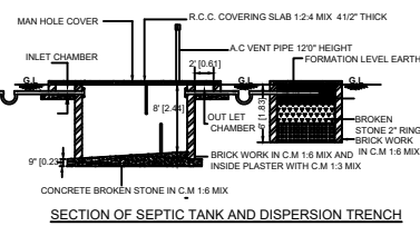
SECTION OF SEPTIC TANK AND DISPERSION TRENCH
