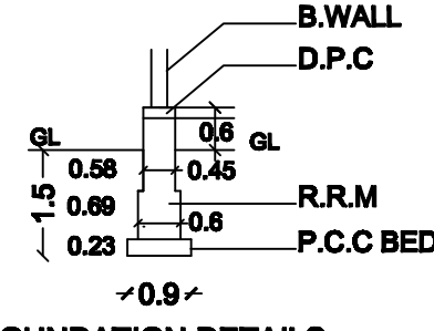
FOUNDATION DETAILS
