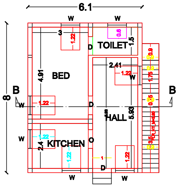
GROUND FLOOR PLAN BLOCK-2
