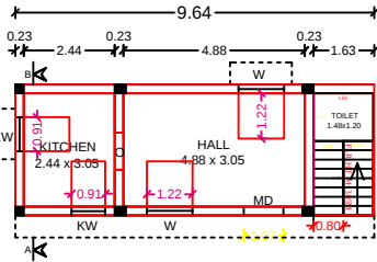
GROUND FLOOR PLAN (EAST FACING)
