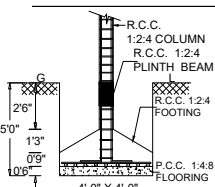
FOUNDATION DETAIL
