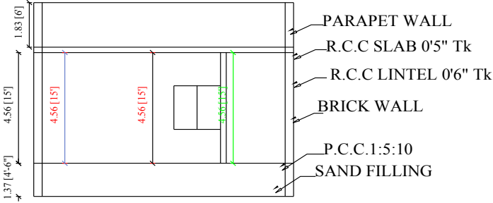
SECTION ON"AB"
