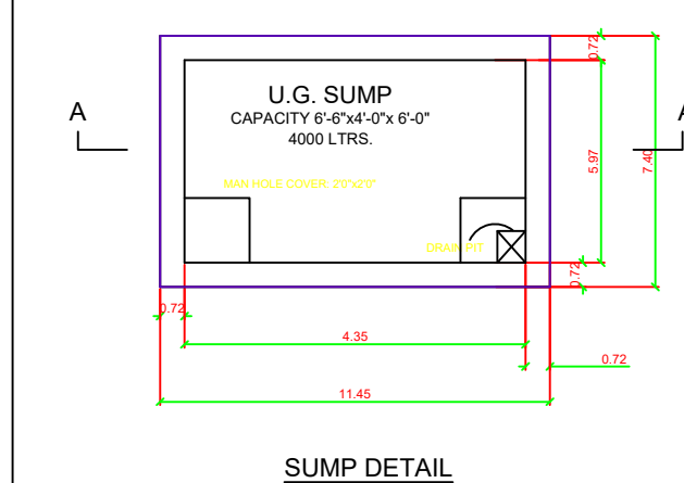
SUMP DETAIL
