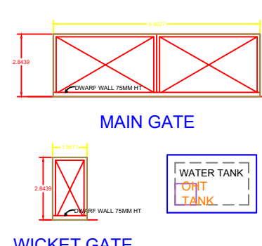
WICKET GATE
