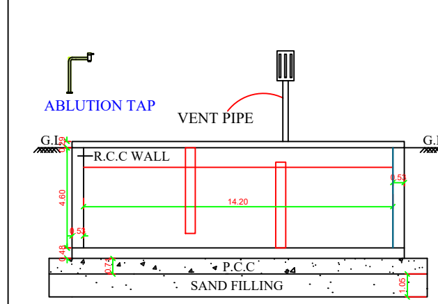
SECTION ON K-B
