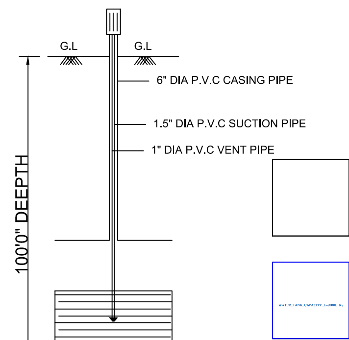
BORE WELL
