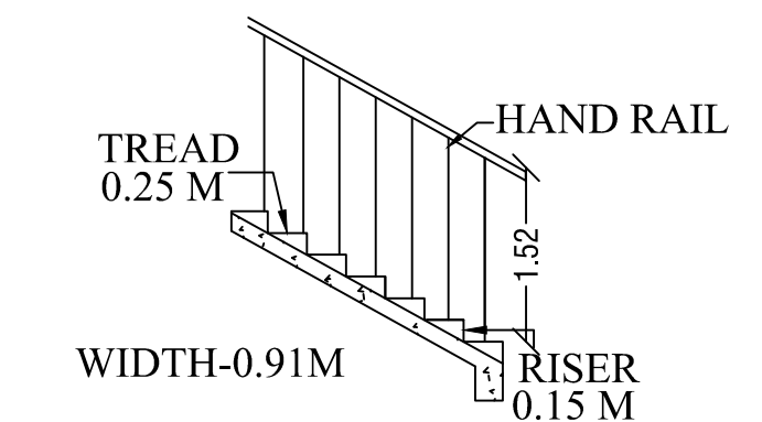
STAIRCASE DETAILS
