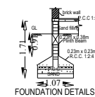
FOUNDATION DETAILS
