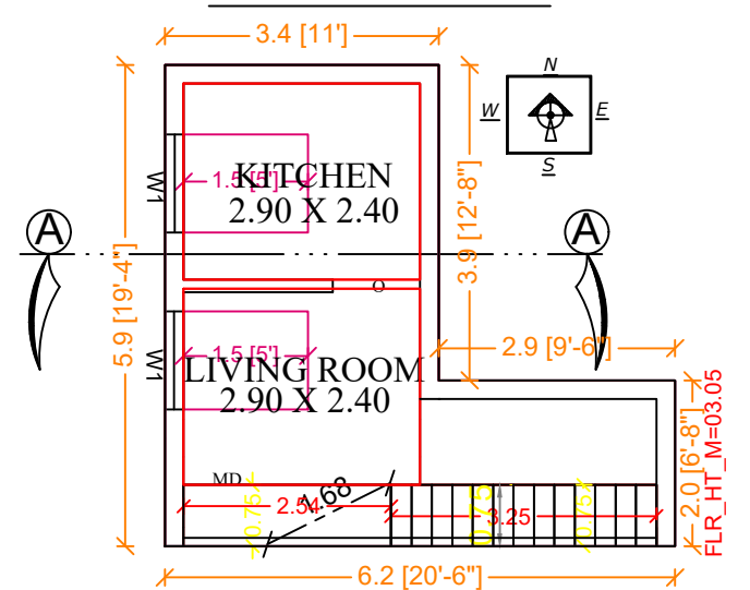
GROUND FLOOR PLAN SINGLE DWELLING UNIT
