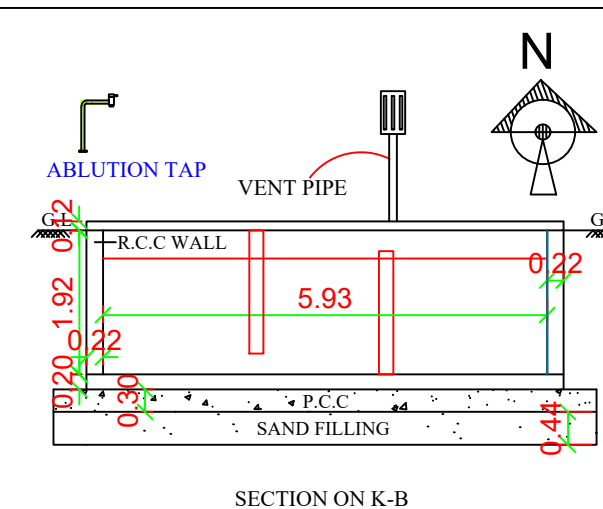
SECTION ON K-B
