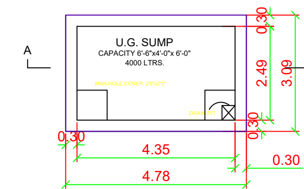
SUMP DETAIL
