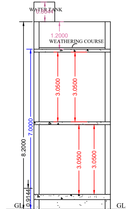
SECTION - 'AA'
