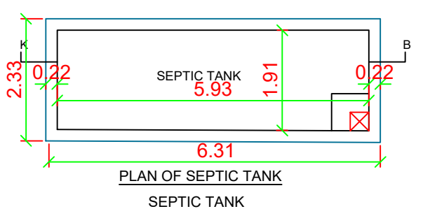
SEPTIC TANK
