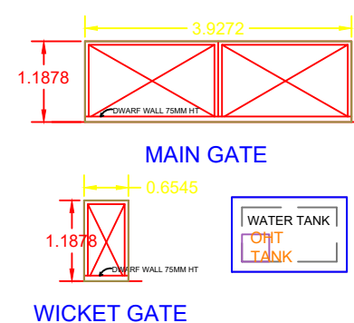
WICKET GATE
