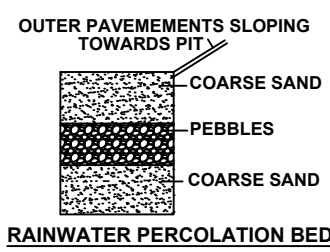
RAINWATER PERCOLATION BED
