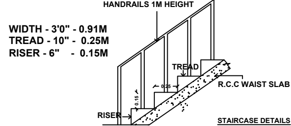
STAIRCASE DETAILS
