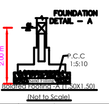
FOUNDATION DETAIL - A (Not to Scale)
