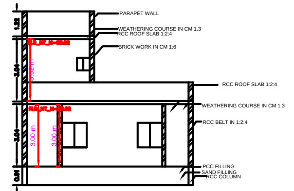
SECTIONON-"AA"&"BB"
