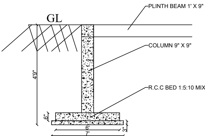
FOOTING DETAILS
