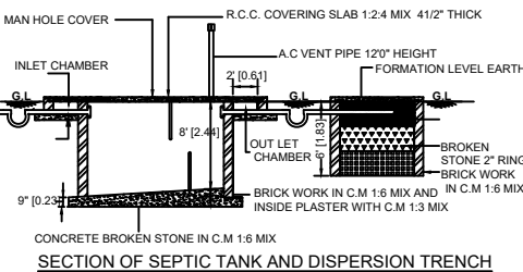
SECTION OF SEPTIC TANK AND DISPERSION TRENCH
