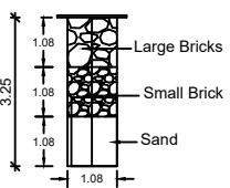
SECTION OF RAIN WATER COLLECTION PITS (NTS)
