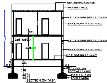
SECTION "AB"
