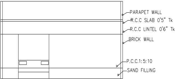
SECTION ON"AB"
