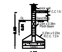
FOUNDATION DETAILS
