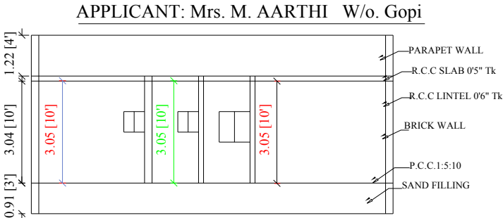
SECTION ON"AB"
