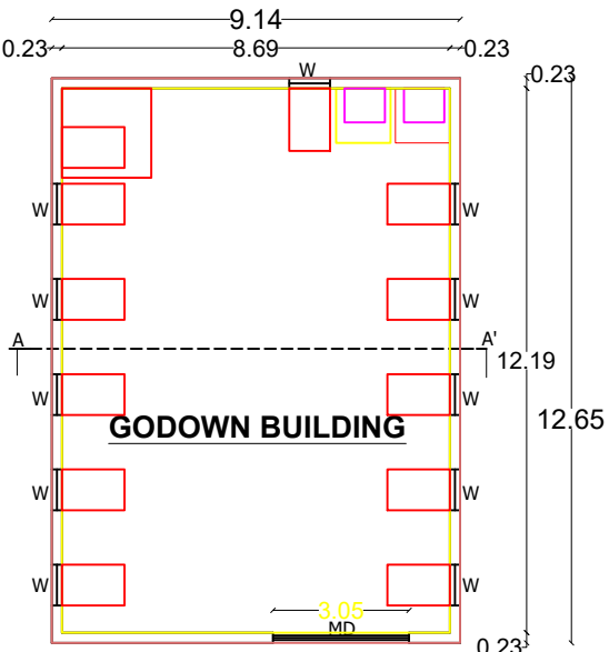
GROUND FLOOR PLAN FACING EAST
