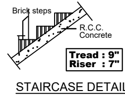
STAIRCASE DETAILS
