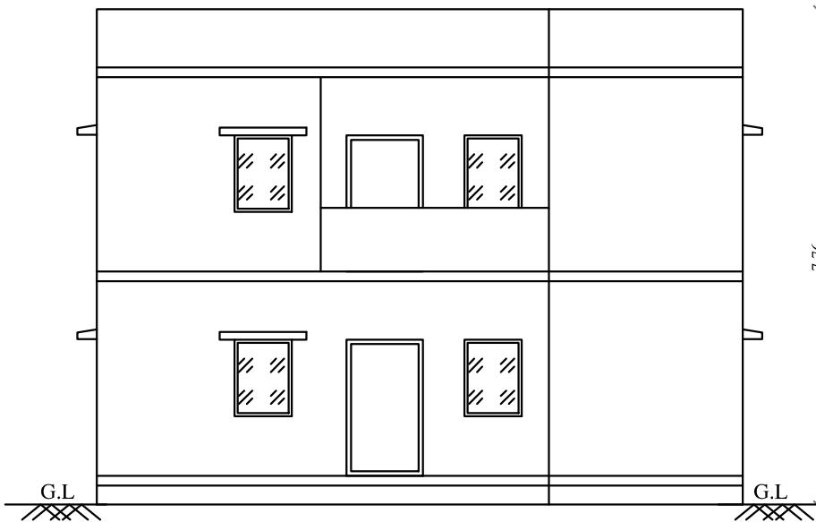
FRONT ELEVATION
