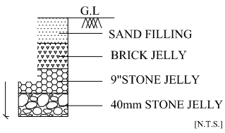
RAIN WATER HARVESTING RECHARGE PIT
