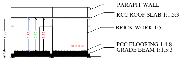
SECTION AB
