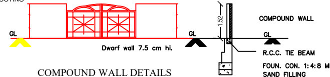
COMPOUND WALL DETAILS
