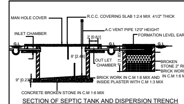
SECTION OF SEPTIC TANK AND DISPERSION TRENCH
