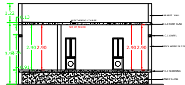
SECTION ON K-S
