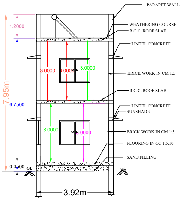
SECTION AB
