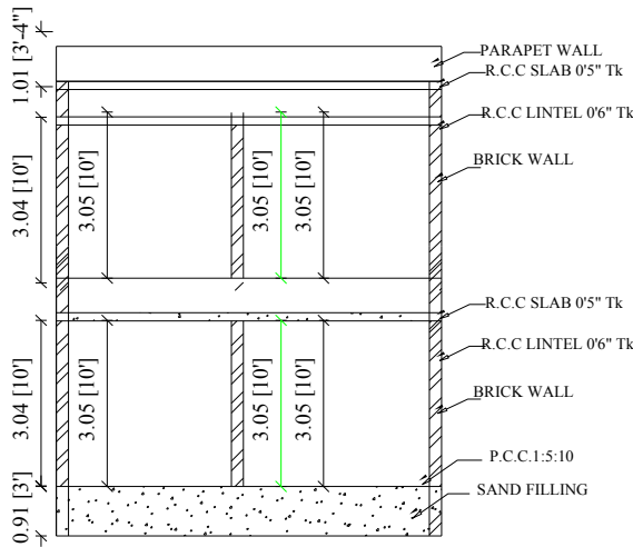
SECTION ON"AB"
