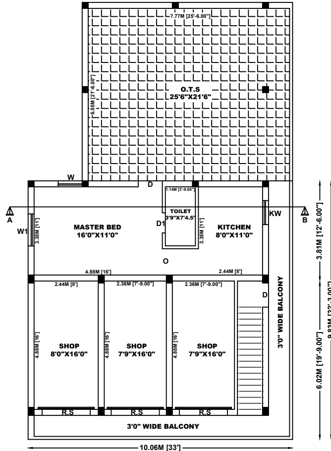
EXISTING&PROPOSED FIRST FLOOR PLAN
