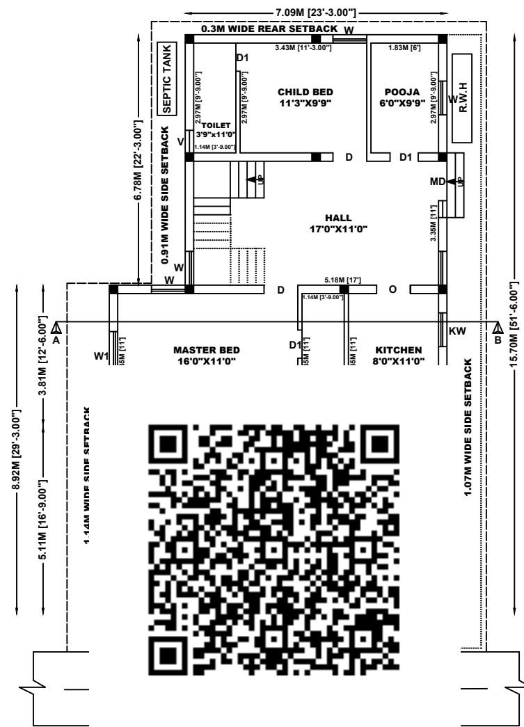
EXISTING&PROPOSED GROUND FLOOR PLAN
