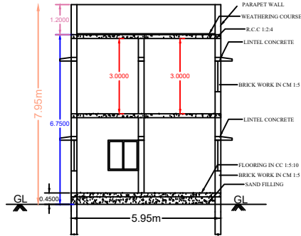
SECTION AB
