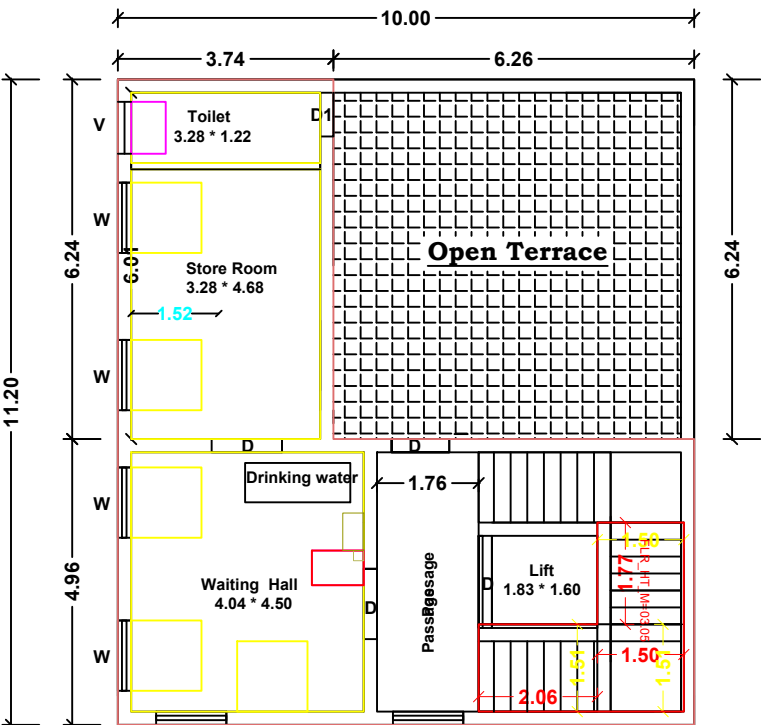
Proposed First Floor - Commercial
