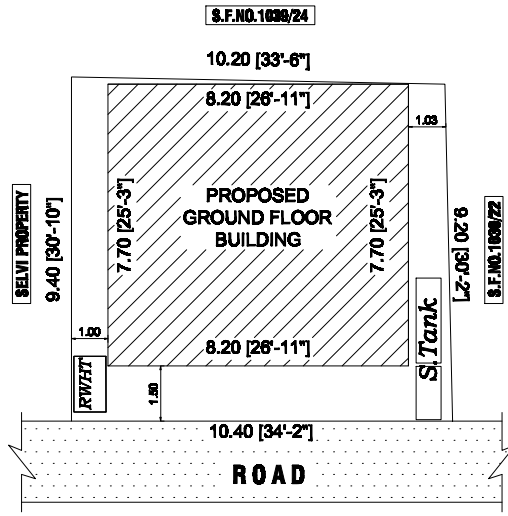
SITE PLAN
