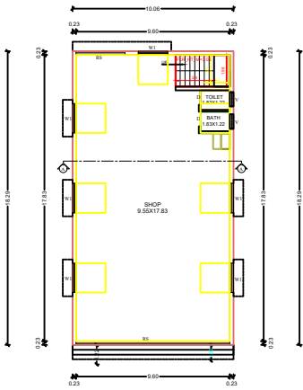
PRO. GROUND FLOOR PLAN (COMMERCIAL)
