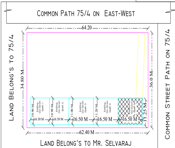
KEY PLAN (As Per Site Location)
