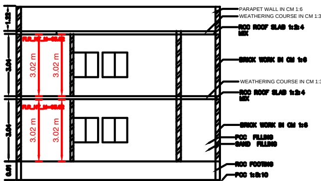
SECTION ON"AB"
