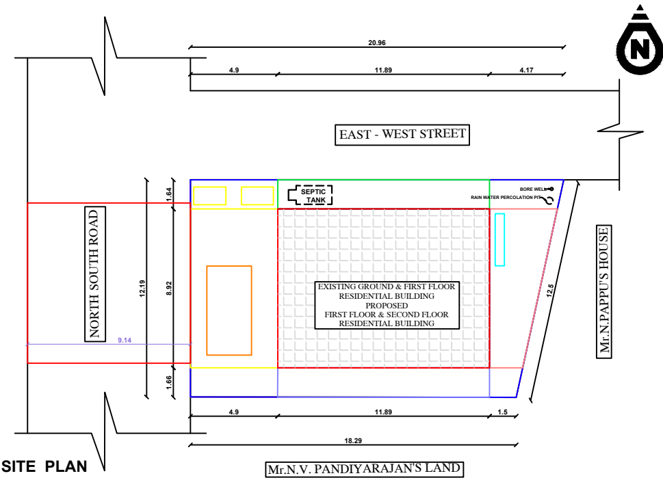
SITE PLAN SCALE : 1 INCH = 8 FEET ( or ) 1 : 100
