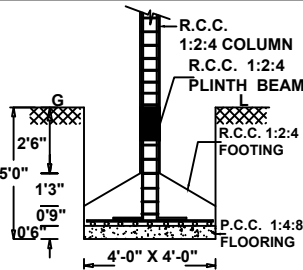
FOUNDATION DETAIL
