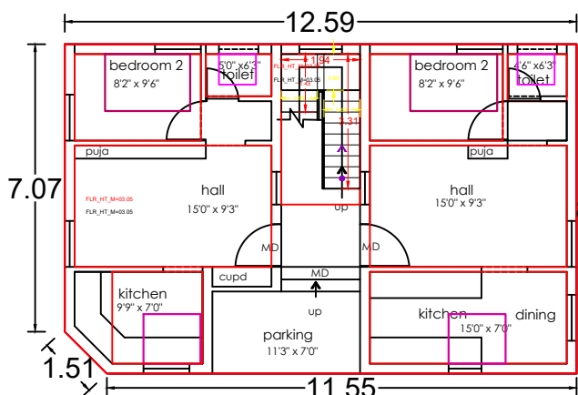
GROUND FLOOR (East Facing)
