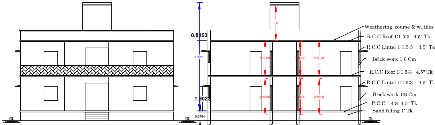
FRONT ELEVATION
