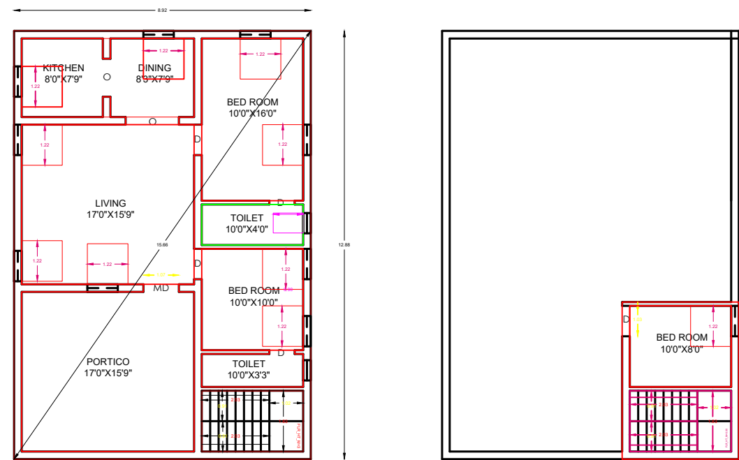
GROUND FLOOR PLAN [NORTH FACING]
