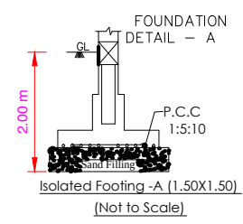
FOUNDATION DETAIL - A
