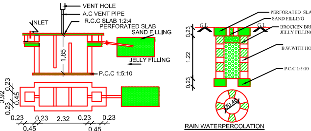
SEPTIC TANK DETAILS
