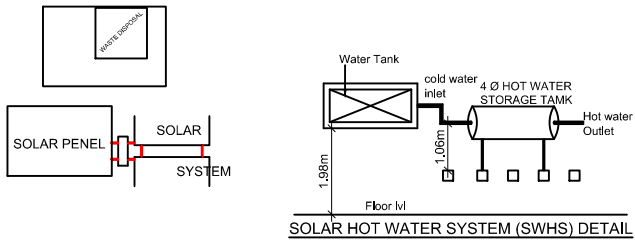
SOLAR HOT WATER SYSTEM (SWHS) DETAIL
