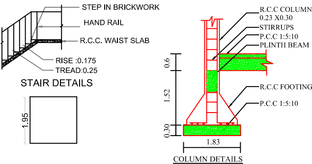
COLUMN DETAILS
