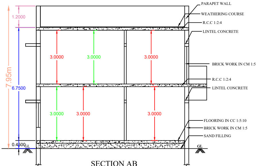
SECTION AB
